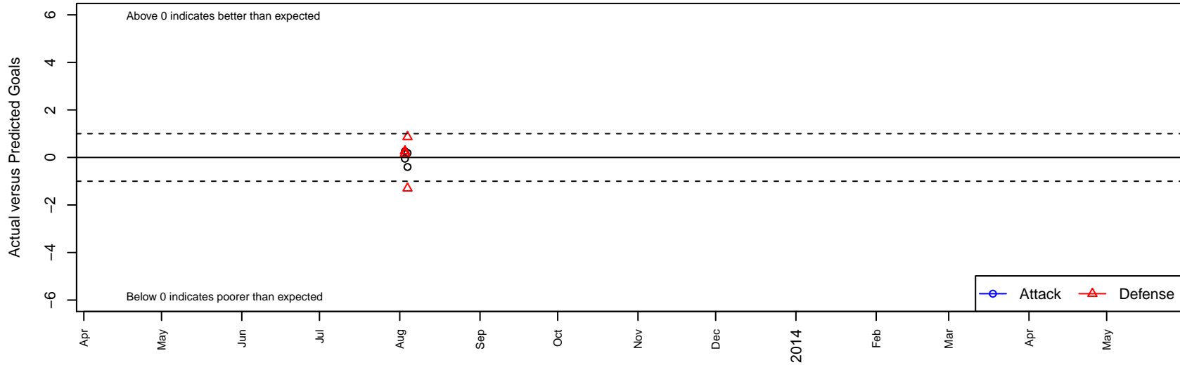
USYS RIV ODP B98 Dots are actual minus expected GF (blue circles) and GA (red triangles). Blue line is smoothed change in attack strength. Red is smoothed change in defense strength.
